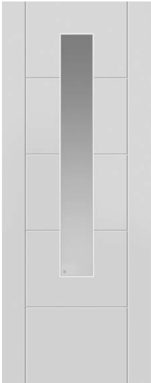
Finished White Composite core Grooved, 5 ladder style panels Pilkington™ opal flat glass double glazed unit U Value 1.6
